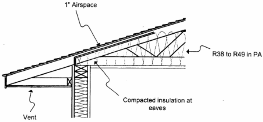
Fig. 1: Typical Insulation Practice on Low-Slope Roofs
