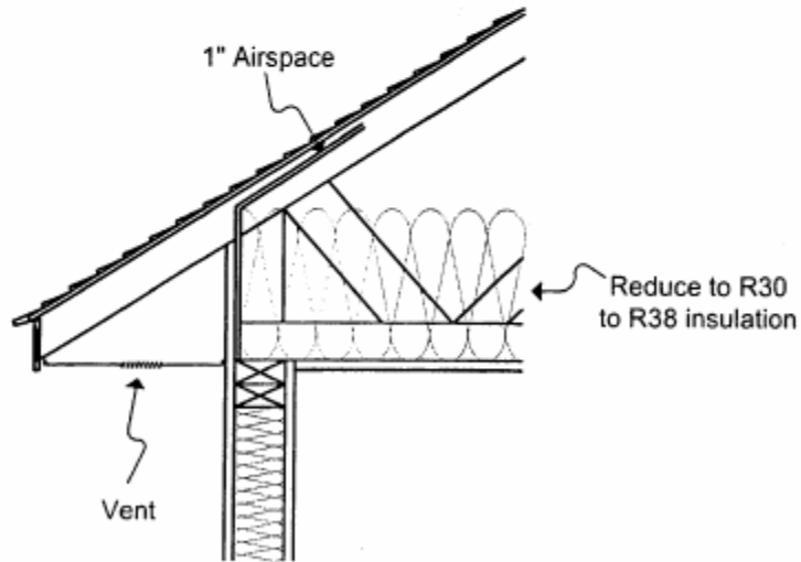
Fig. 2: Raised-Heal Truss
